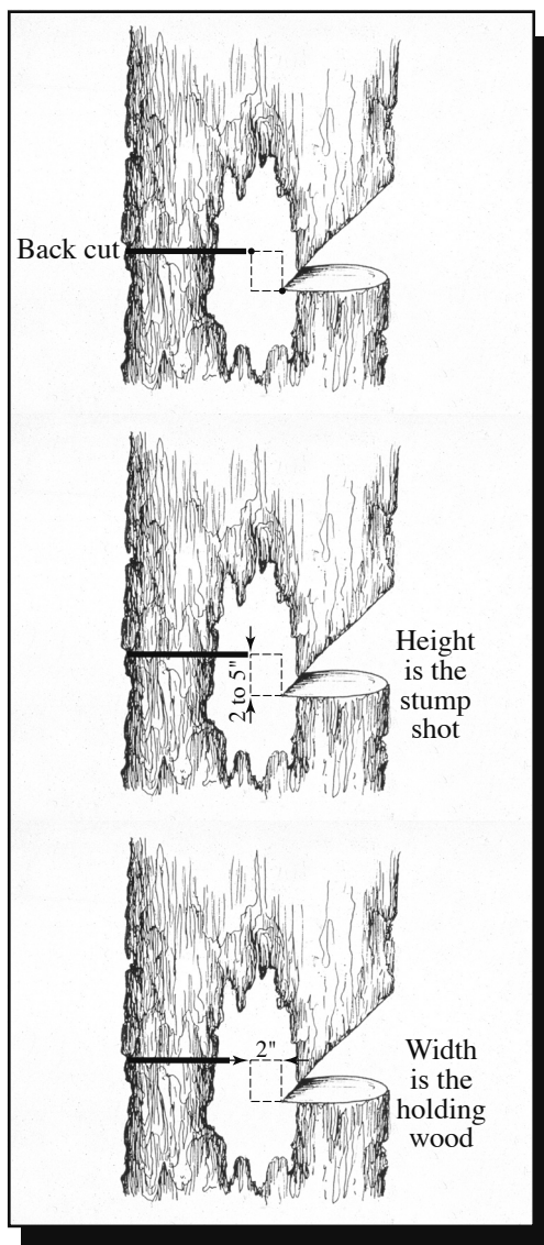
Figure 60—An imaginary rectangle can help the sawyer understand the importance of the back cut.
