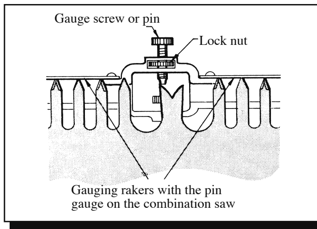
Figure 22—Gauging rakers.
