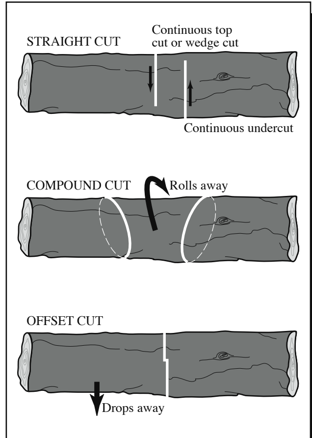
Figure 47—Three basic cuts: straight, compound, and offset.
