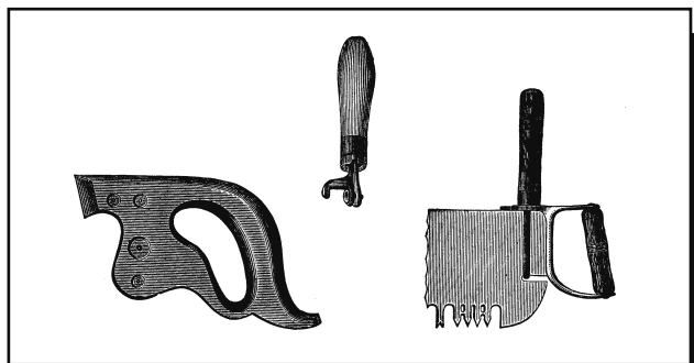
Figure 16—One-person saw “D” handle and supplemental handles from a vintage Disston catalog.—Henry Disston & Sons, Inc., catalog (1902), with permission of Astragal Press, Mendham, NJ
