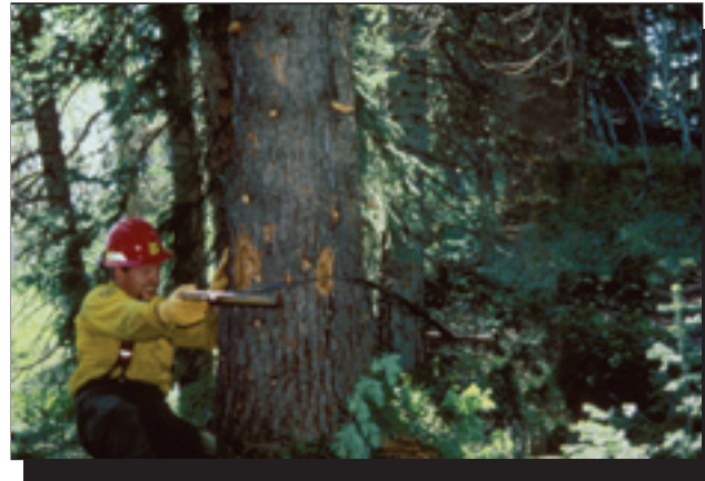
Figure 5-29—Gunning the saw helps determine the specific direction of the undercut. (Photo has been digitally altered to remove distracting items.)
