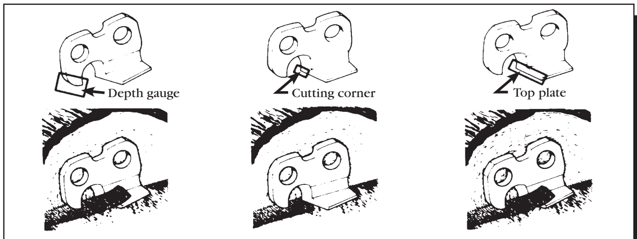
Figure 3-9—The depth gauge controls the depth at which a tooth's cutting corner bites into the wood.—Oregon Maintenance and Safety Manual, permission by Blount, Inc.
